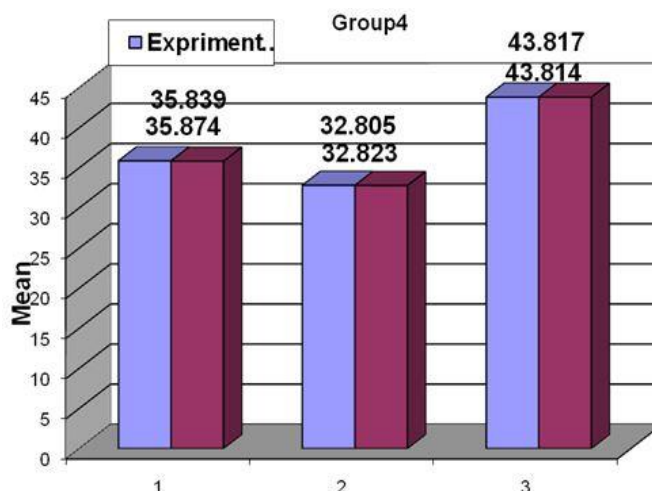
Fig (10) Mean values of dimensional stability among tested group (Experimental) in (mm)
